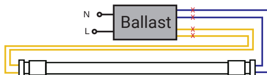
Step 1 Cut off the wires and remove the ballast
